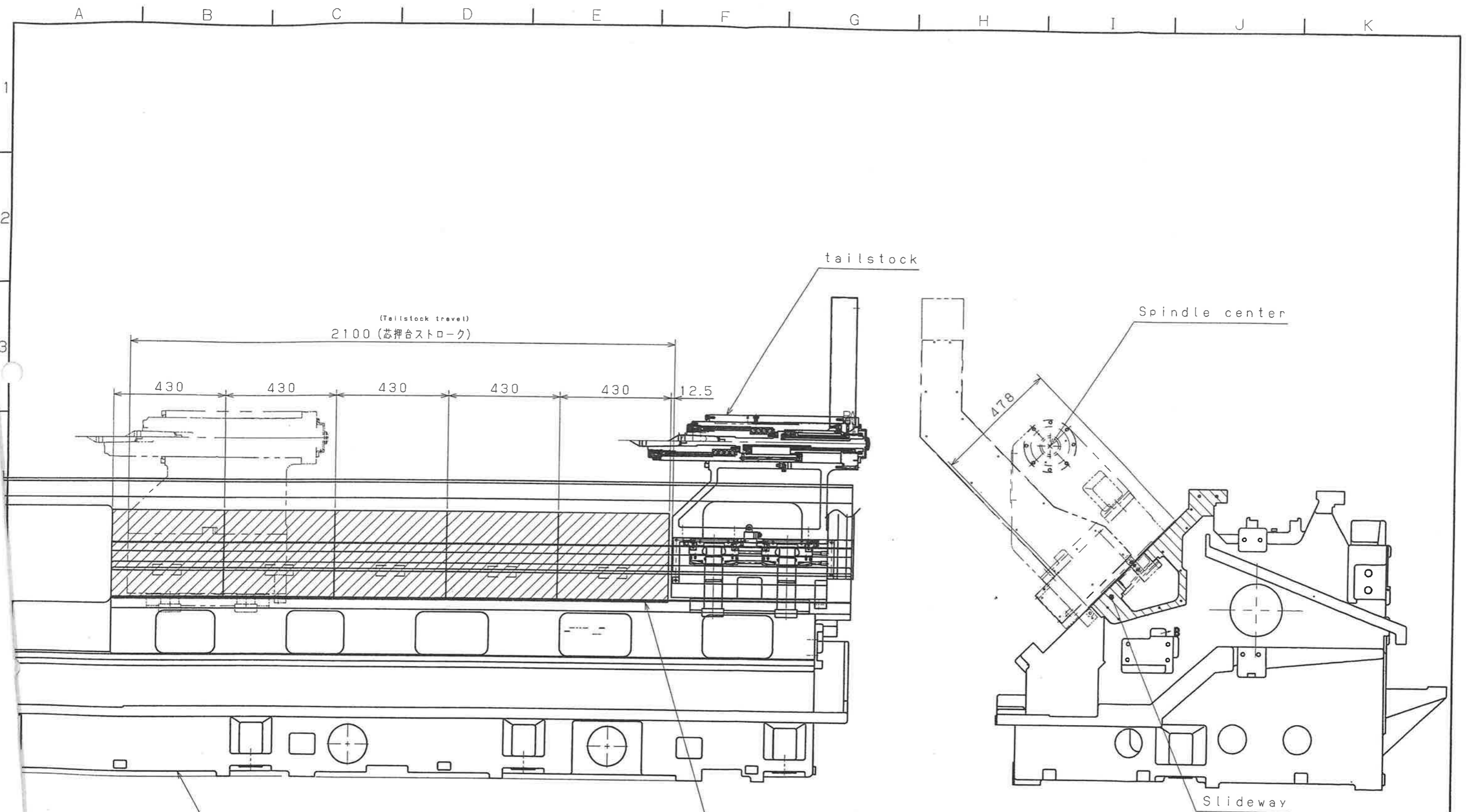
Protective cover for slideway 5-摺動面保護カバー (430x478、t=1.6)
